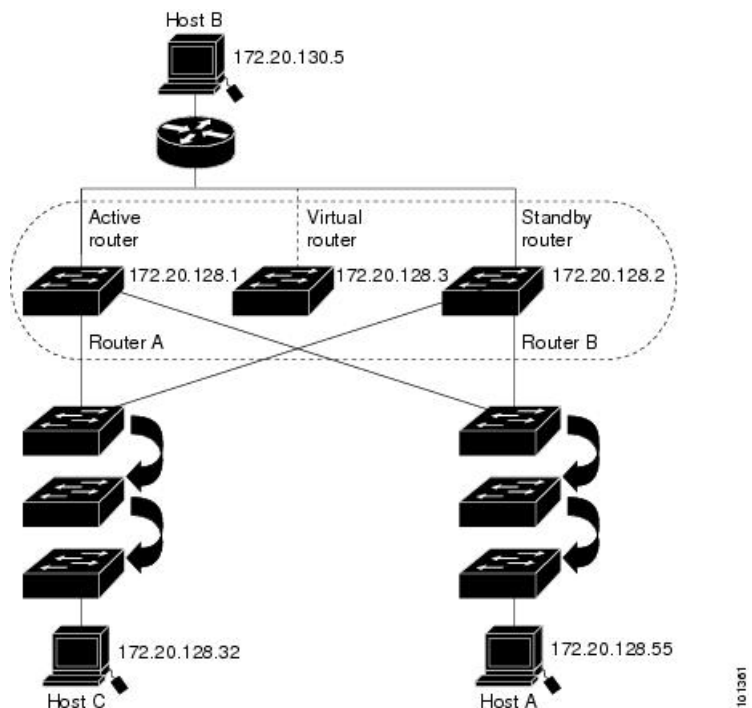
Figure 1: Typical HSRP Configuration
