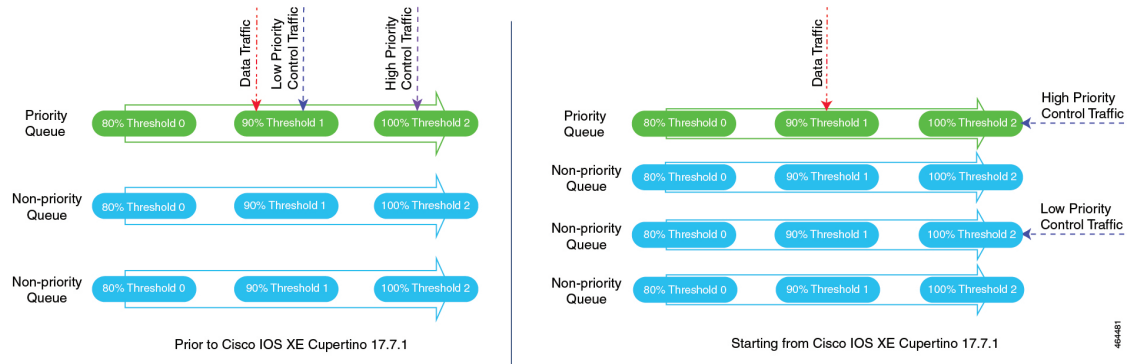
Figure 3: Traffic Mapping to a Priority Queue
