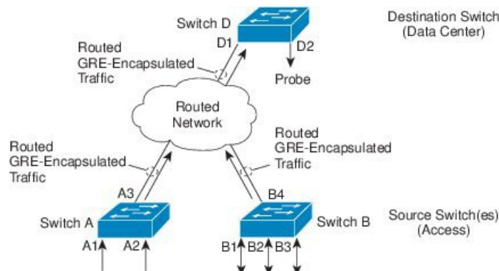
Figure 10: ERSPAN Configuration
