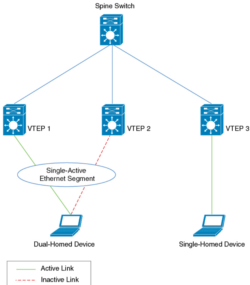
Figure 2: Dual-Homed Device Topology
