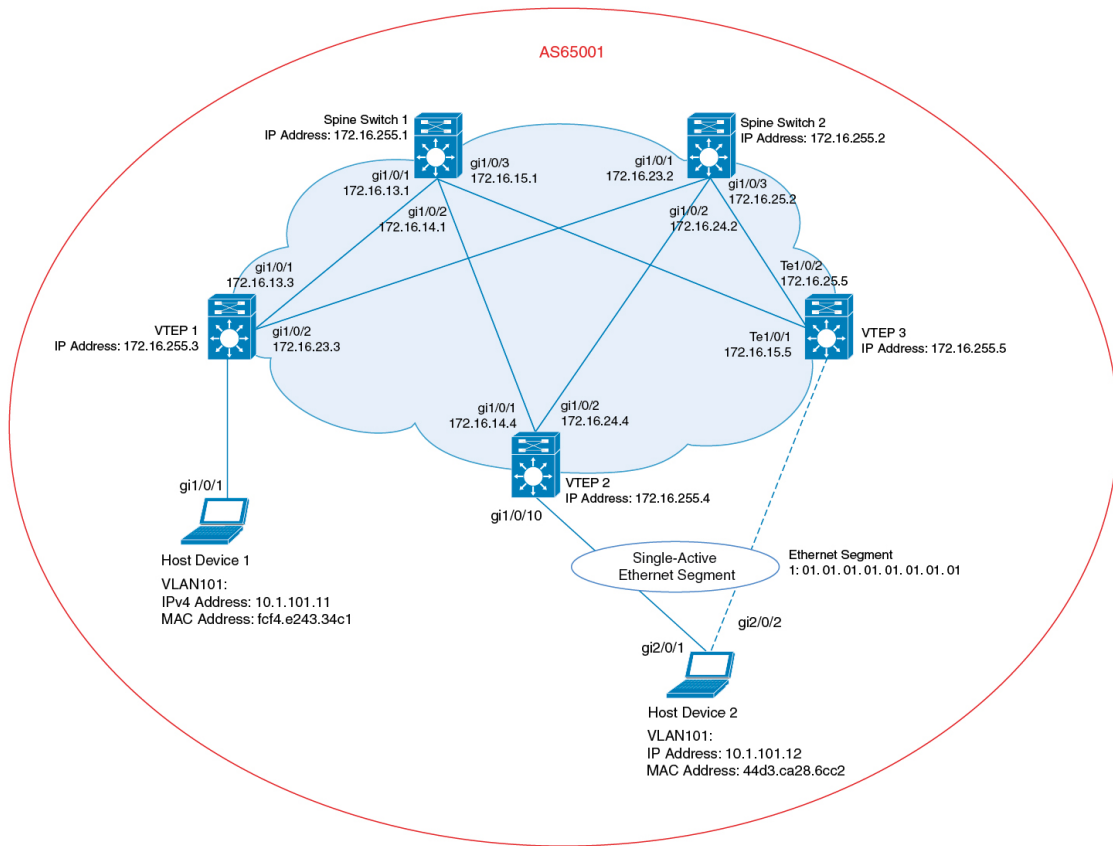
Figure 6: Dual-Homing with Single-Active Redundancy in a BGP EVPN VXLAN Fabric
