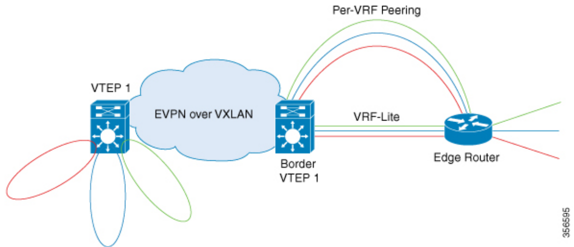
Figure 3: Layer 3 External Connectivity with VRF-Lite
