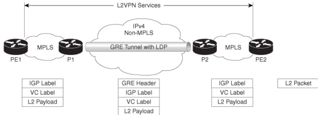
Figure 3: P-to-P Tunneling
