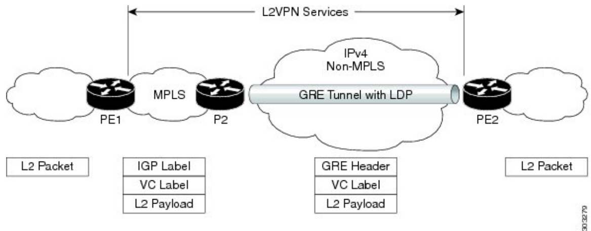
Figure 2: P-to-PE Tunneling
