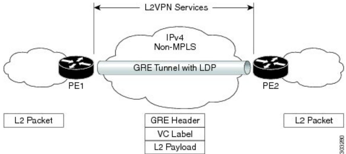
Figure 1: PE-to-PE Tunneling
