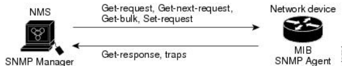
Figure 1: SNMP Network
