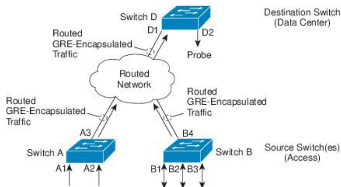
Figure 10: ERSPAN Configuration
