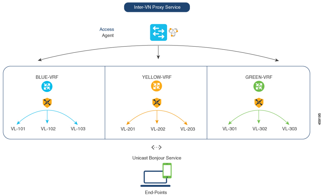
Figure 25: Inter-VN Proxy Service
