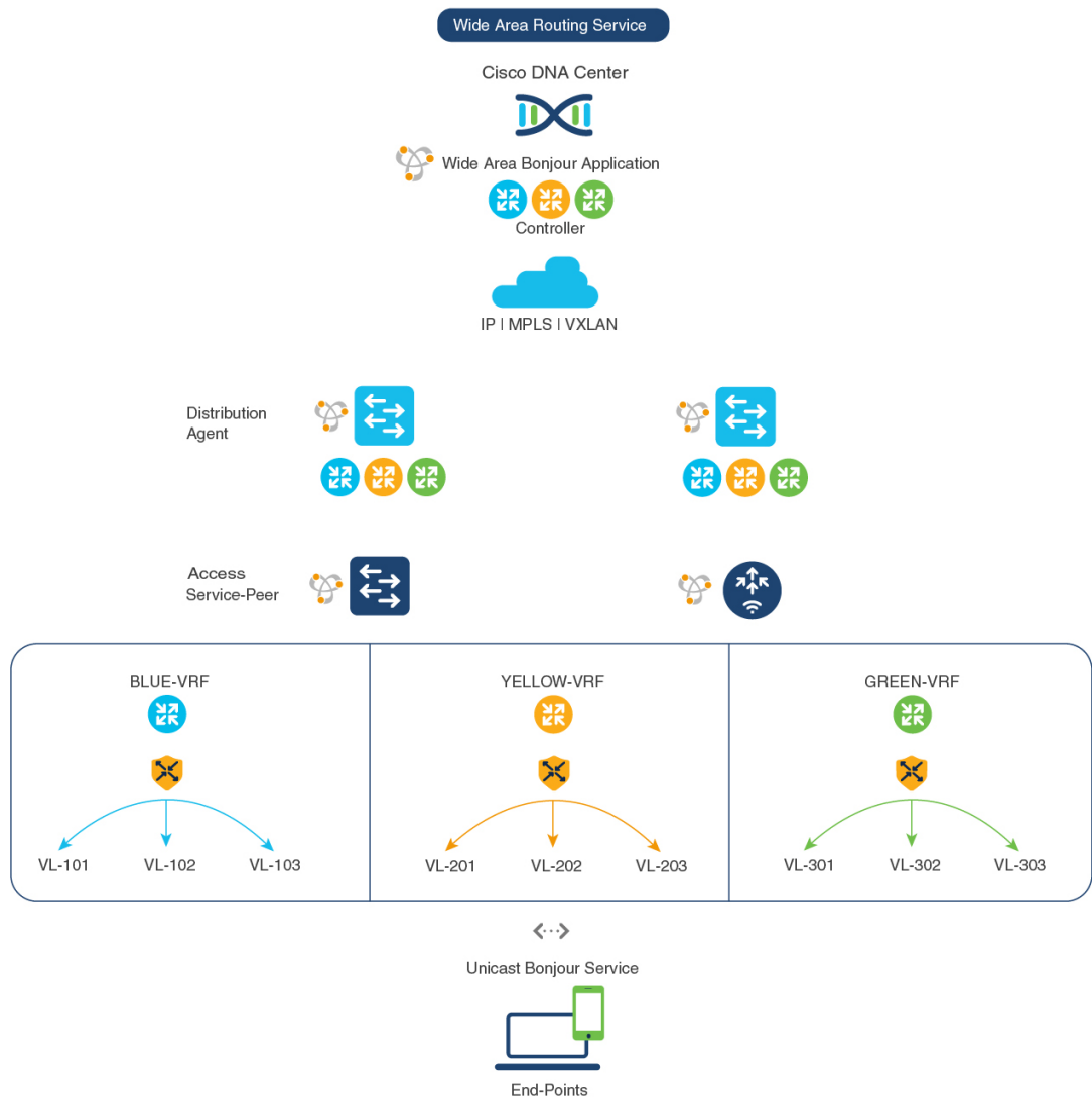
Figure 23: VRF-Aware on Multilayered Wired and Wireless Network
