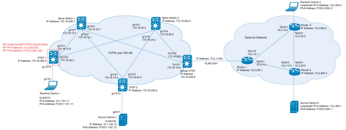
Figure 43: TRM with PIM-SM when the RP is Inside the BGP EVPN VXLAN Fabric
