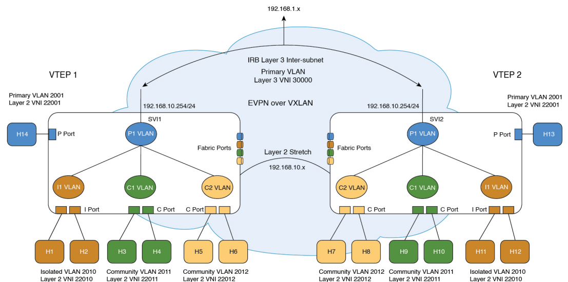
Figure 59: PVLAN Extension in a BGP EVPN VXLAN Fabric
