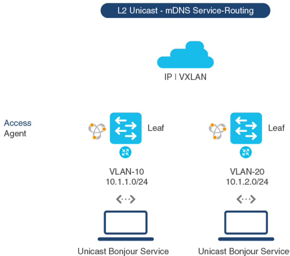
Figure 88: Layer 3 BGP EVPN Leaf Access SDG Agents
