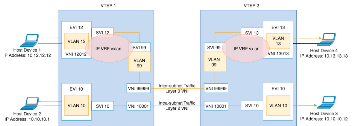
Figure 75: Movement of traffic in an EVPN VXLAN network Through Layer 2 and Layer 3 VNIs
