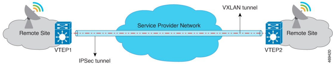
Figure 68: Secure VXLAN Traffic Between Two VTEPs
