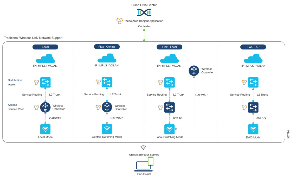
Figure 80: Enterprise Traditional Wireless LAN Network Design
