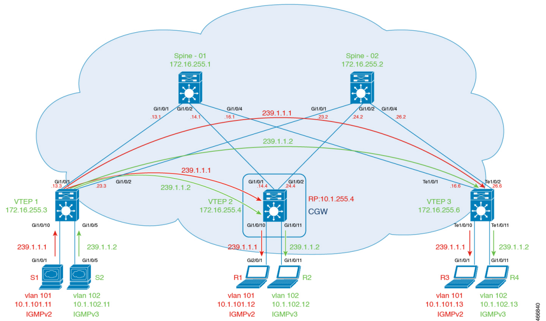
Figure 26: Topology for Optimized Layer 2 Overlay Multicast for IPv4 Traffic with Ingress Replication
