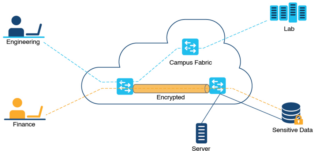
Figure 67: Campus LAN With Secure BGP EVPN VXLAN Network
