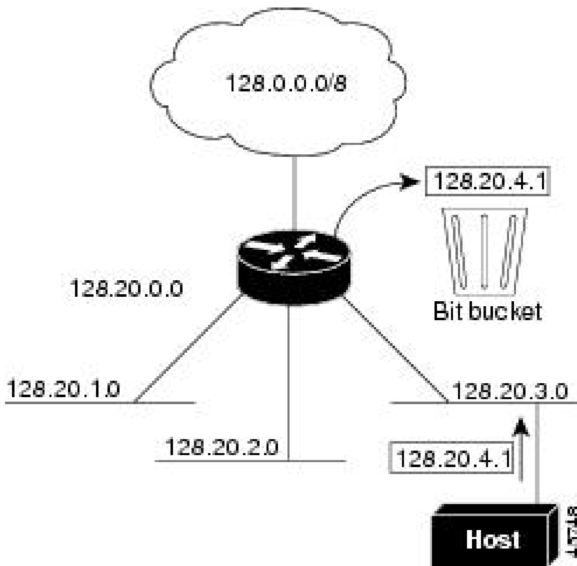
Figure 6: No IP Classless Routing
