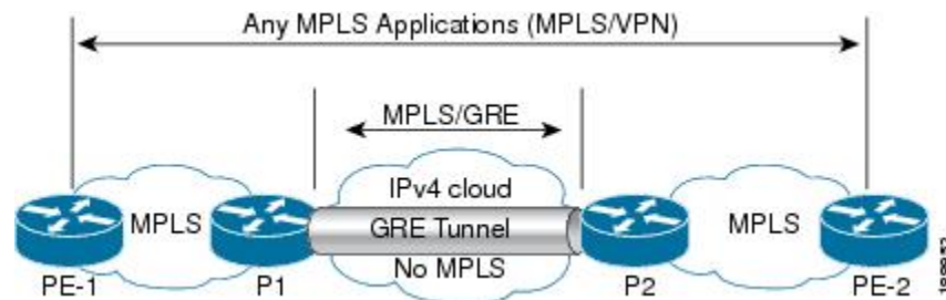
Figure 12: P-to-P Tunneling
