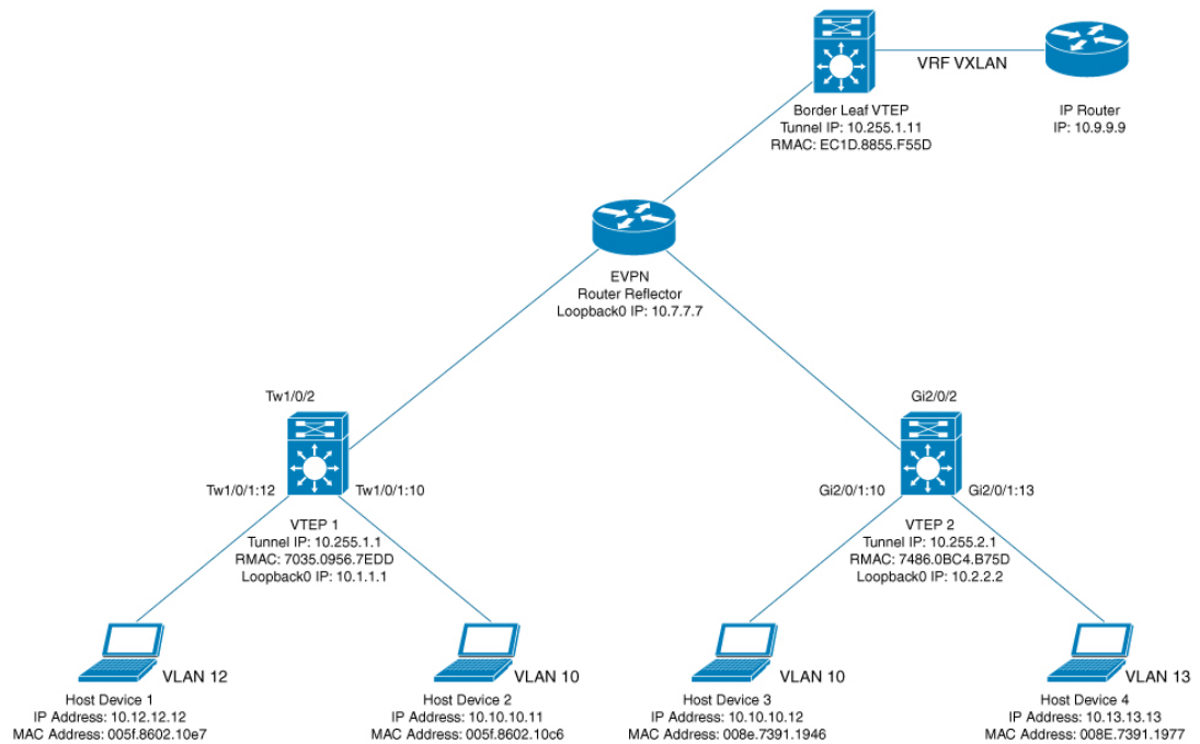
Figure 70: EVPN VXLAN Topology
