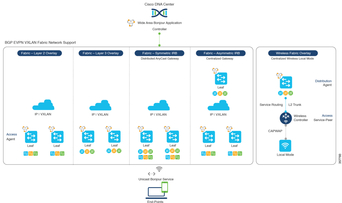
Figure 80: BGP EVPN VXLAN Wired and Wireless Design Alternatives
