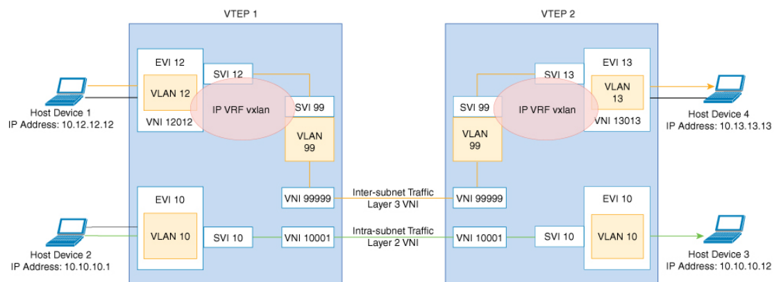
Figure 71: Movement of traffic in an EVPN VXLAN network Through Layer 2 and Layer 3 VNIs
