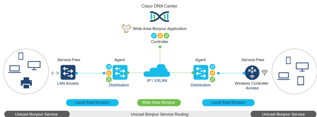
Figure 79: Overlay Bonjour Service for a BGP EVPN-Enabled Enterprise Network
