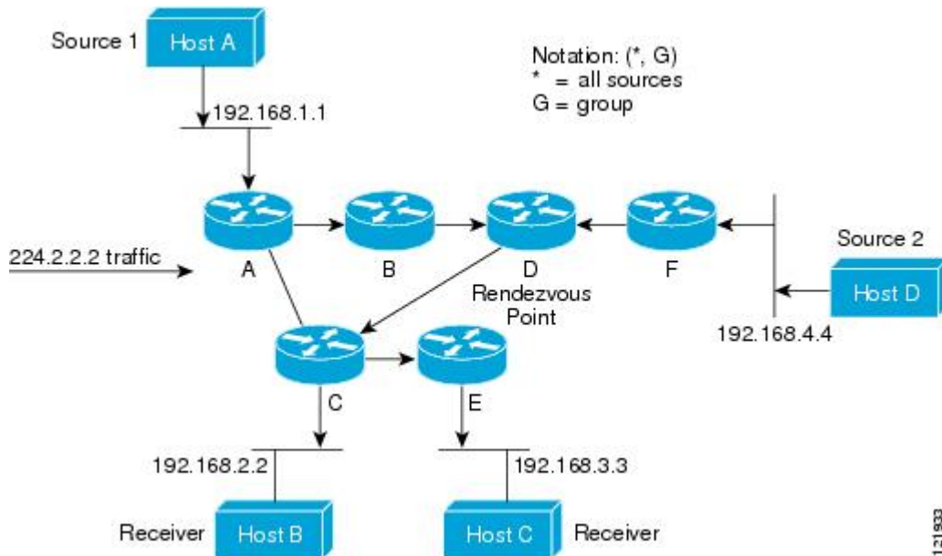
Figure 3: Shared Tree
