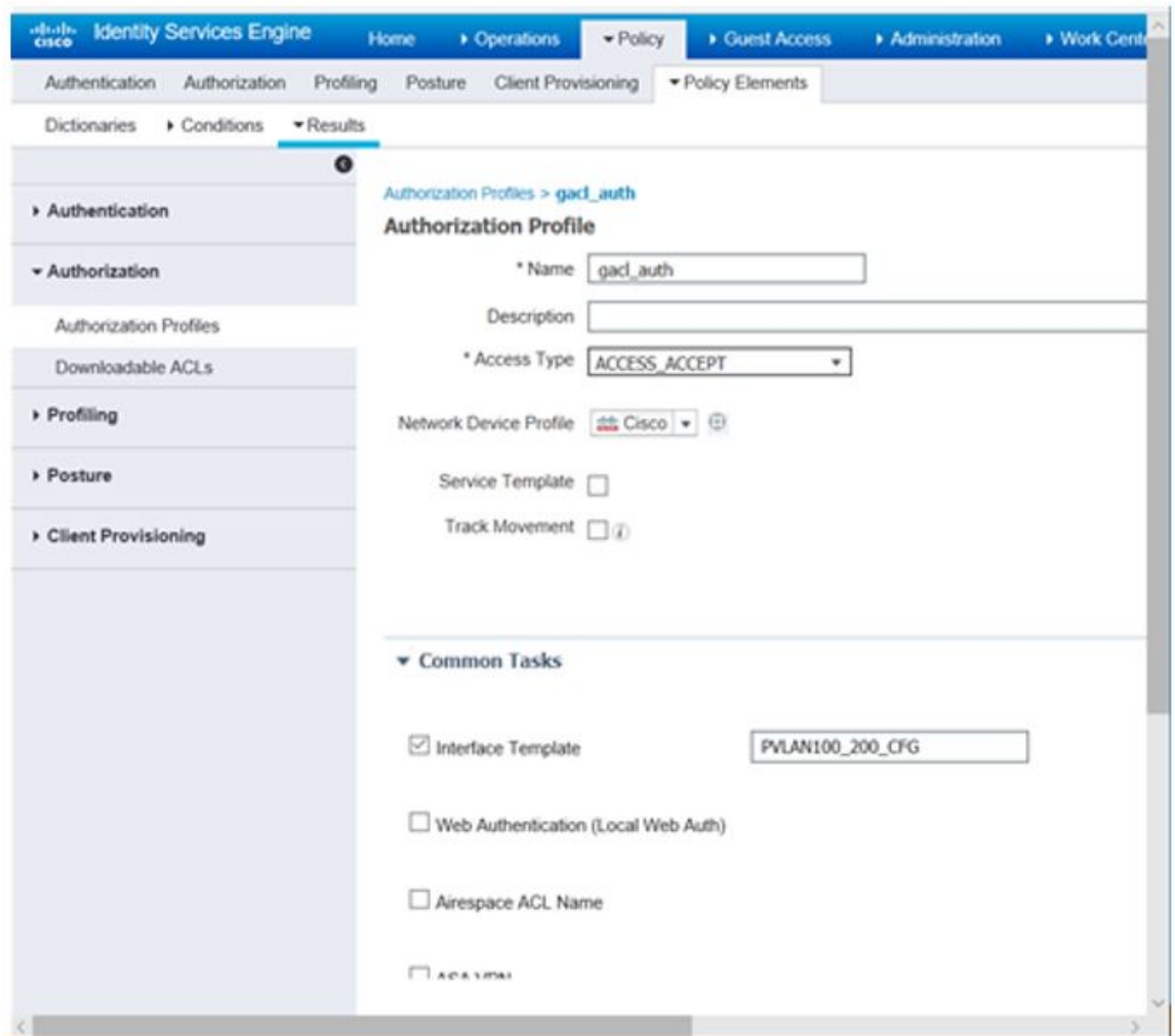
Figure 1: Configuring the ISE to Assign the Interface Template
