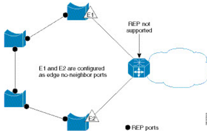
Figure 25: Edge No-Neighbor Ports
