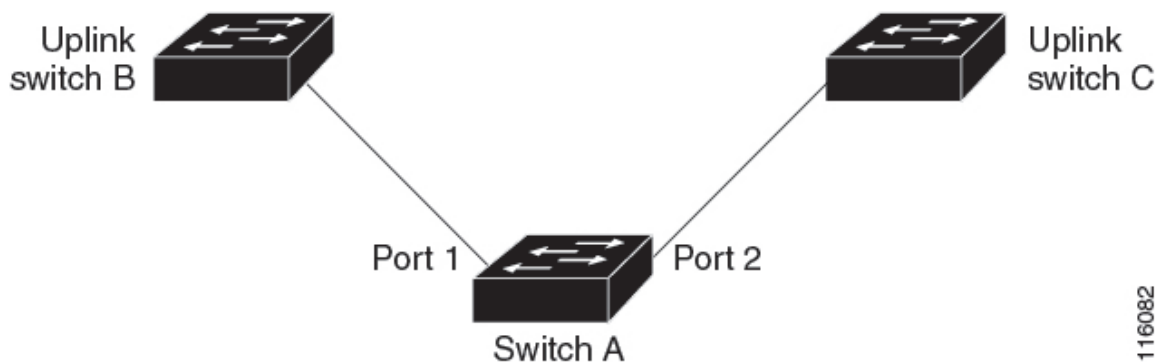
Figure 35: FlexLink+ Topology
