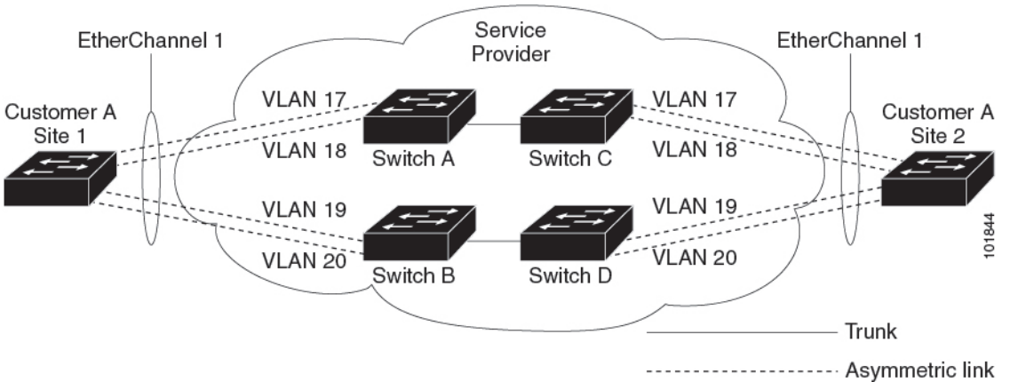
Figure 29: Layer 2 Protocol Tunneling for EtherChannels
