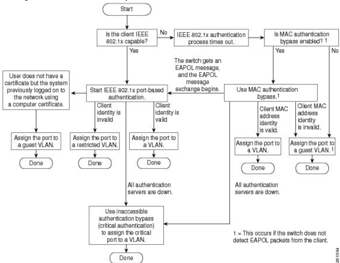
Figure 36: Authentication Flowchart
