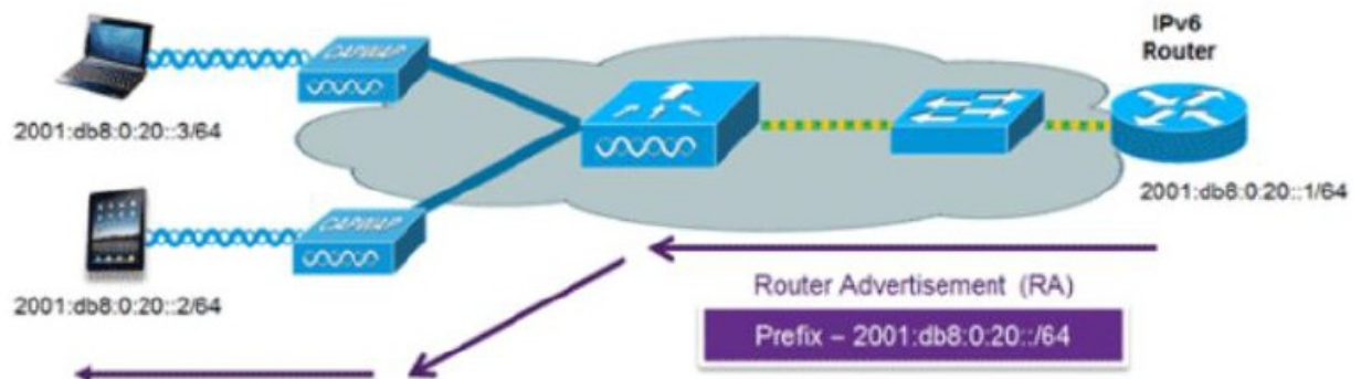
Figure 2: SLAAC Address Assignment
