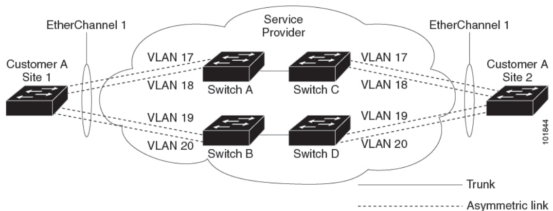
Figure 27: Layer 2 Protocol Tunneling for EtherChannels
