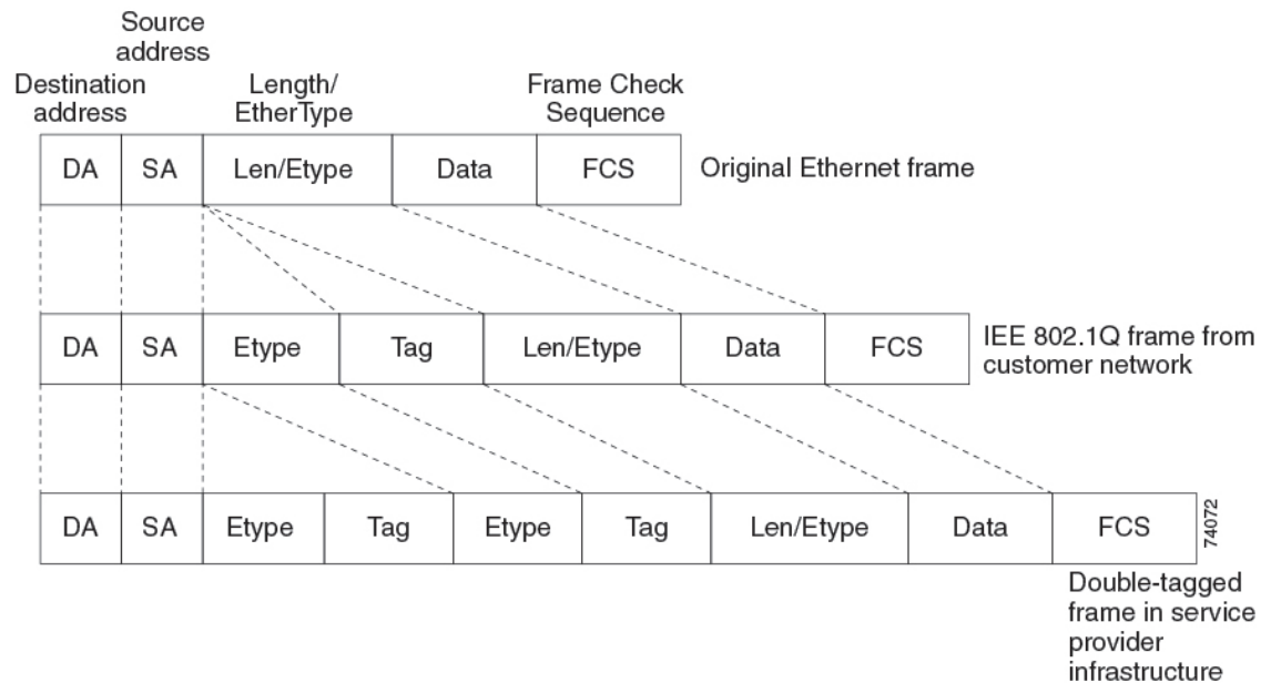
Figure 29: Original (Normal), IEEE 802.1Q, and Double-Tagged Ethernet Packet Formats
