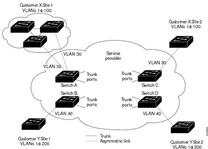
Figure 25: Layer 2 Protocol Tunneling
