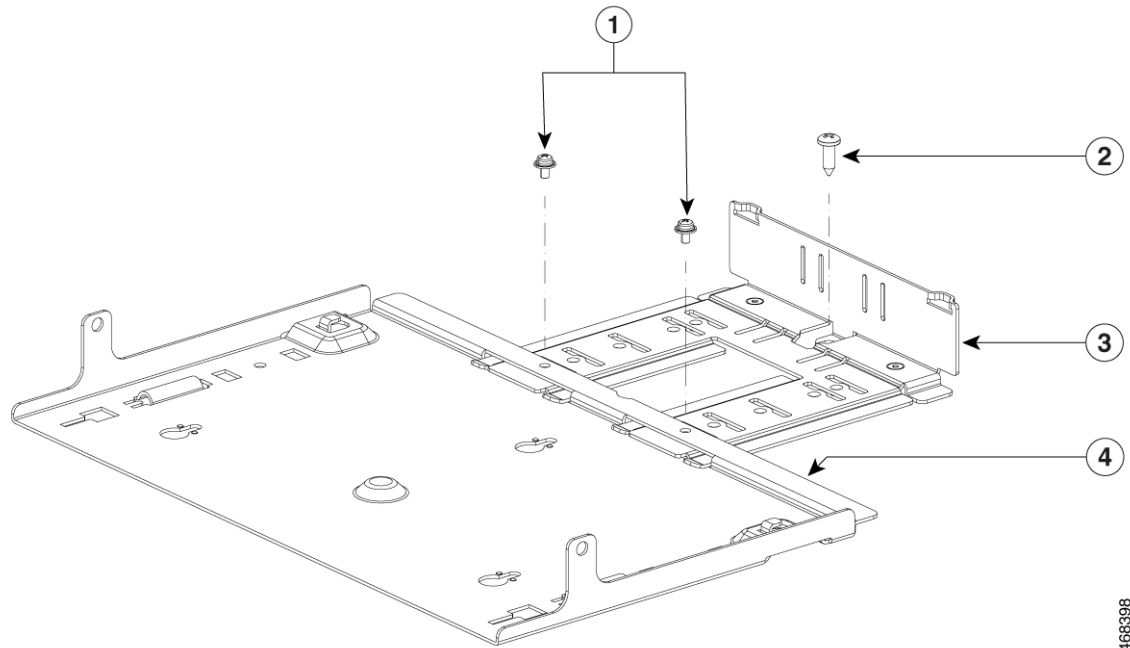
Figure 19: Attaching the Power Adapter Bracket
