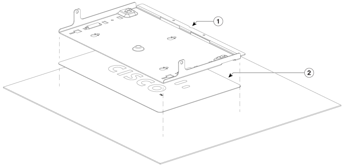
Figure 5: Placing the Mounting Tray on the Magnet
