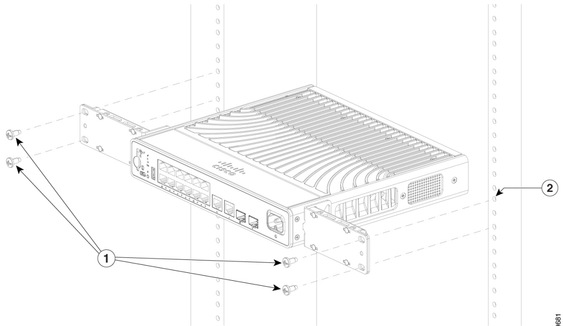
Figure 13: Attaching the Brackets to the Rack
