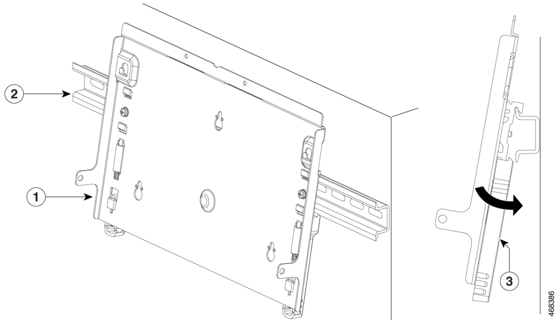
Figure 14: Attaching the DIN Rail Mount to the DIN Rail
