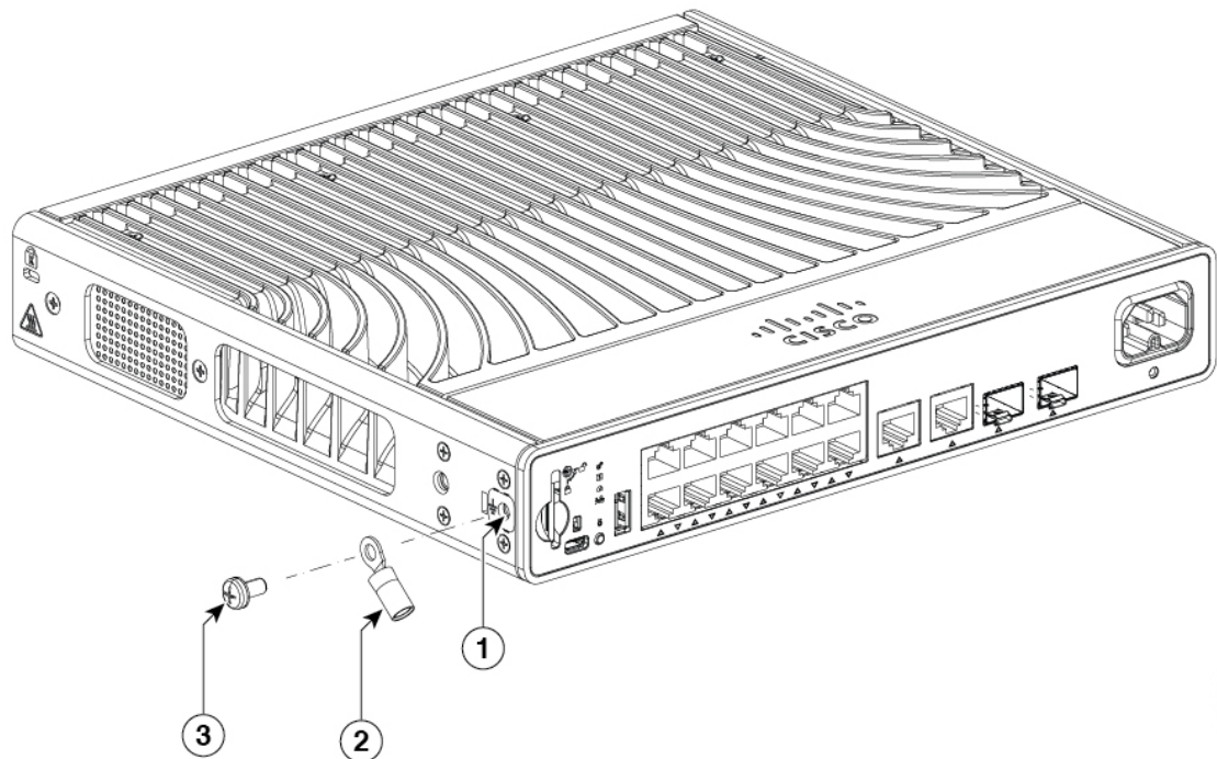
Figure 17: Attaching the Grounding Lug
