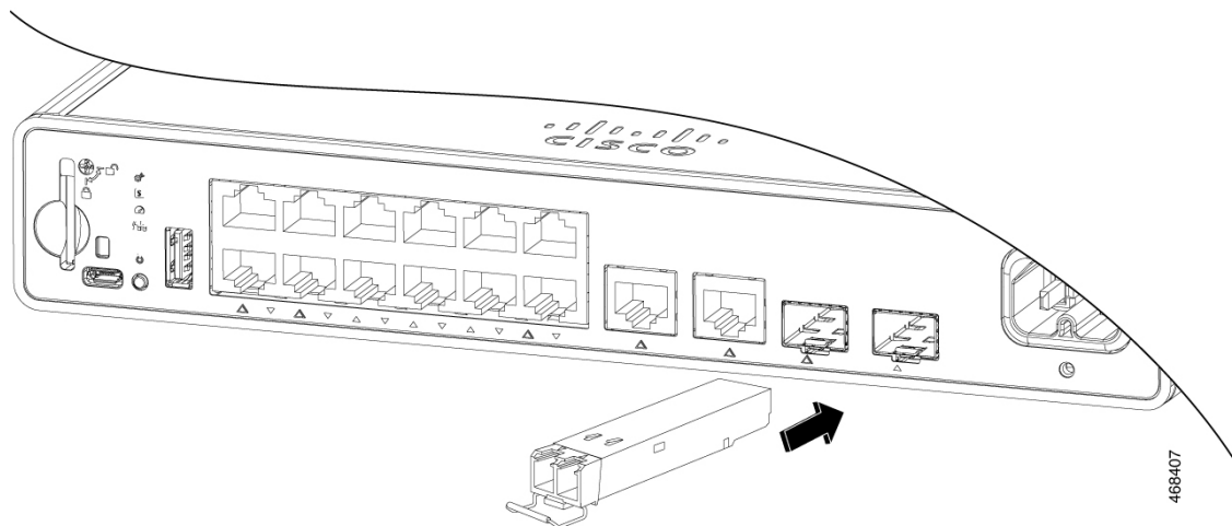
Figure 27: Installing an SFP Module
