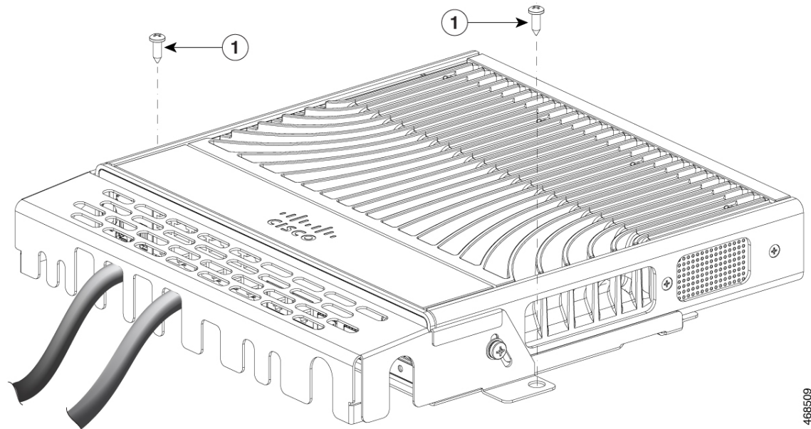
Figure 26: Switch with Cable Guide Installed
