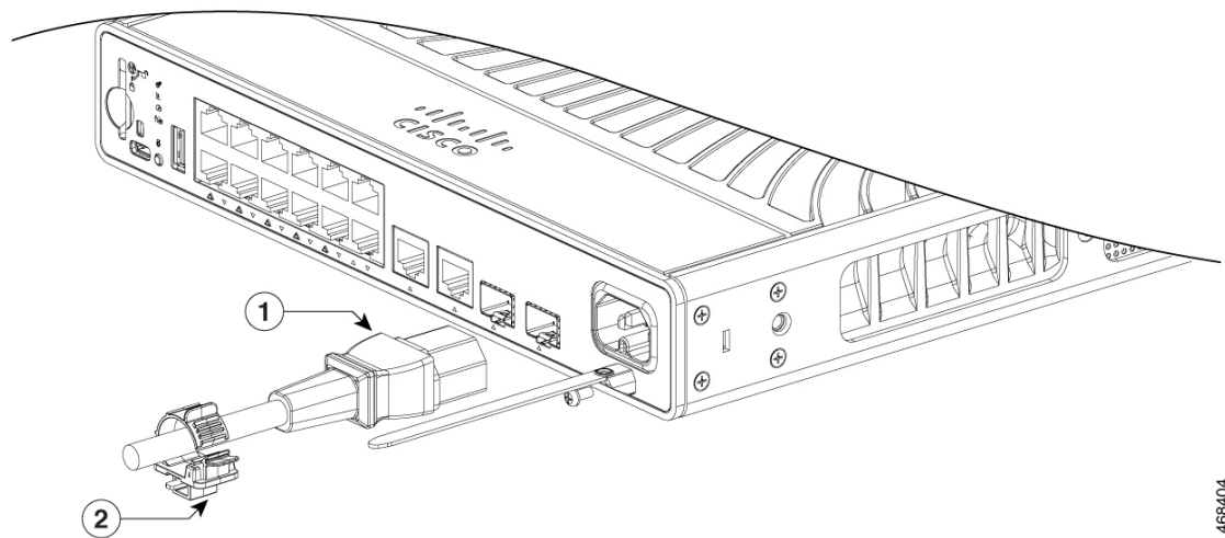
Figure 22: Sliding the Retainer Clamp Through the Power Cord
