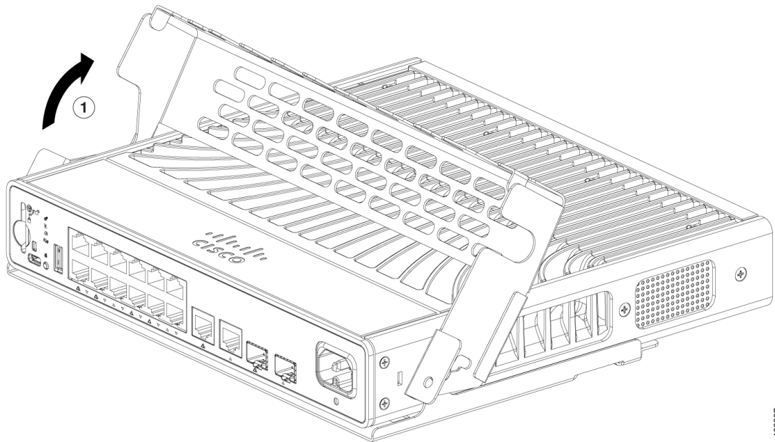
Figure 25: Pivoting the Cable Guard Upwards
