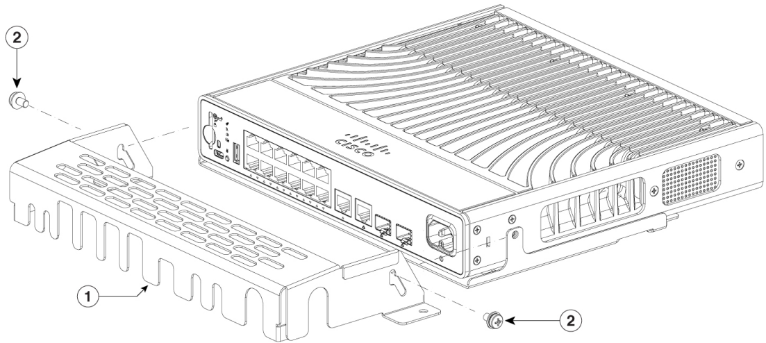
Figure 24: Attaching the Cable Guard to the Switch
