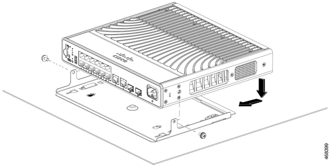
Figure 7: Securing the Switch to the Mounting Tray
