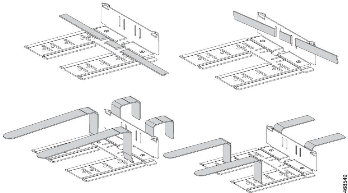
Figure 18: Threading the Velcro Strap through the Adapter Bracket
