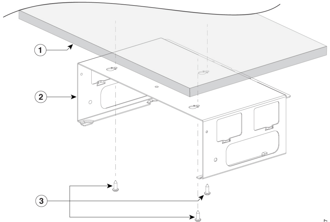
Figure 8: Installing the Desk Mount Under a Desk or a Shelf
