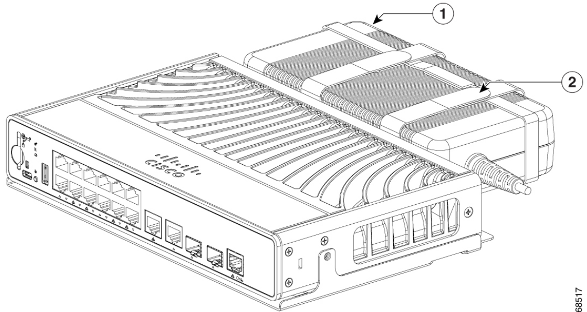
Figure 20: Securing the Power Adapter to the Adapter Bracket
