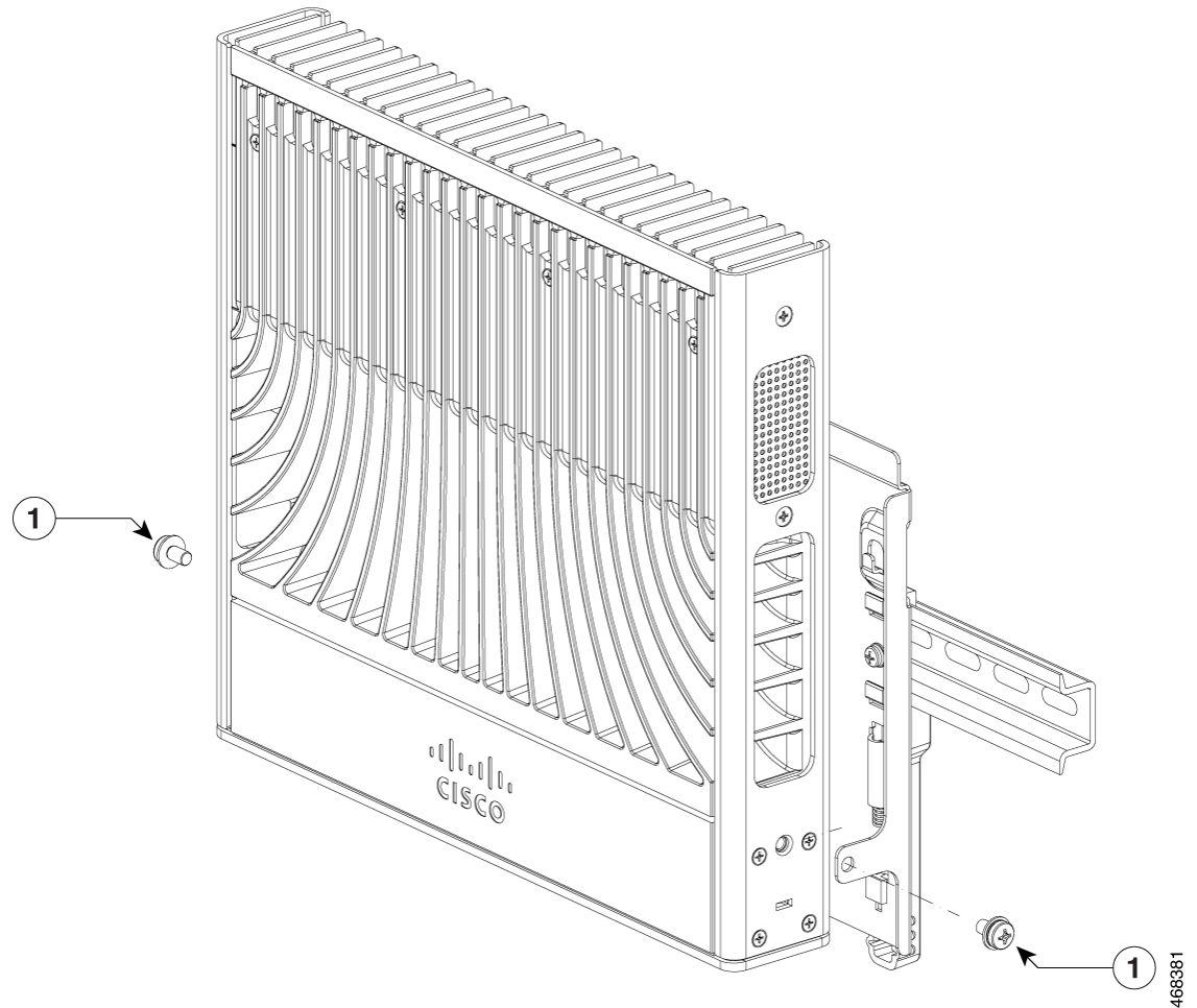
Figure 15: Securing the Switch to the DIN Rail
