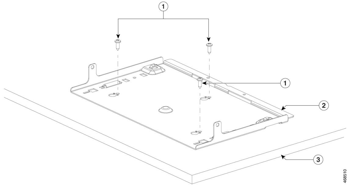
Figure 2: Attaching the Mounting Tray to the Desk or Shelf
