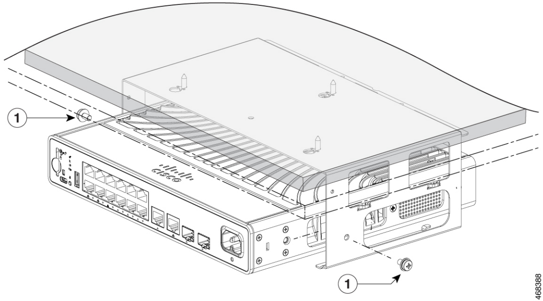
Figure 10: Mounting the Switch Under a Desk or Shelf
