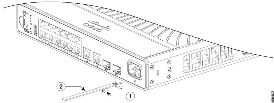
Figure 21: Attaching the Power Cord Retainer Strap
