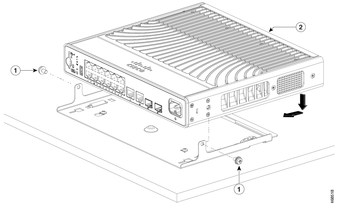
Figure 4: Securing the Switch to the Mounting Tray
