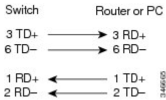
Figure 8: Two Twisted-Pair Crossover Cable Schematic
