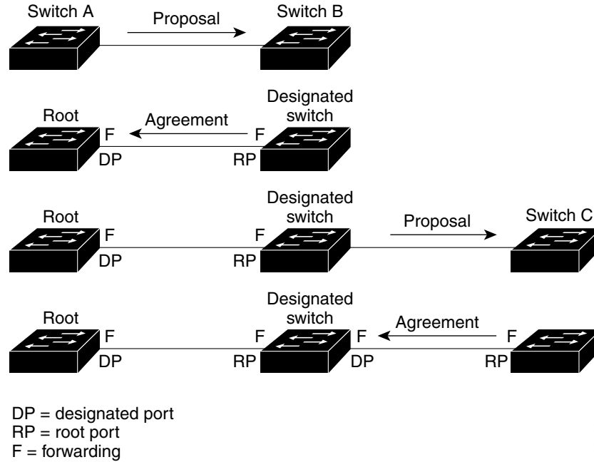
Figure 30-8 Proposal and Agreement Handshaking for Rapid Convergence
