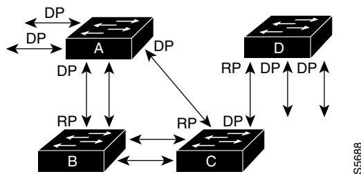
Figure 30-1 Spanning Tree Topology
