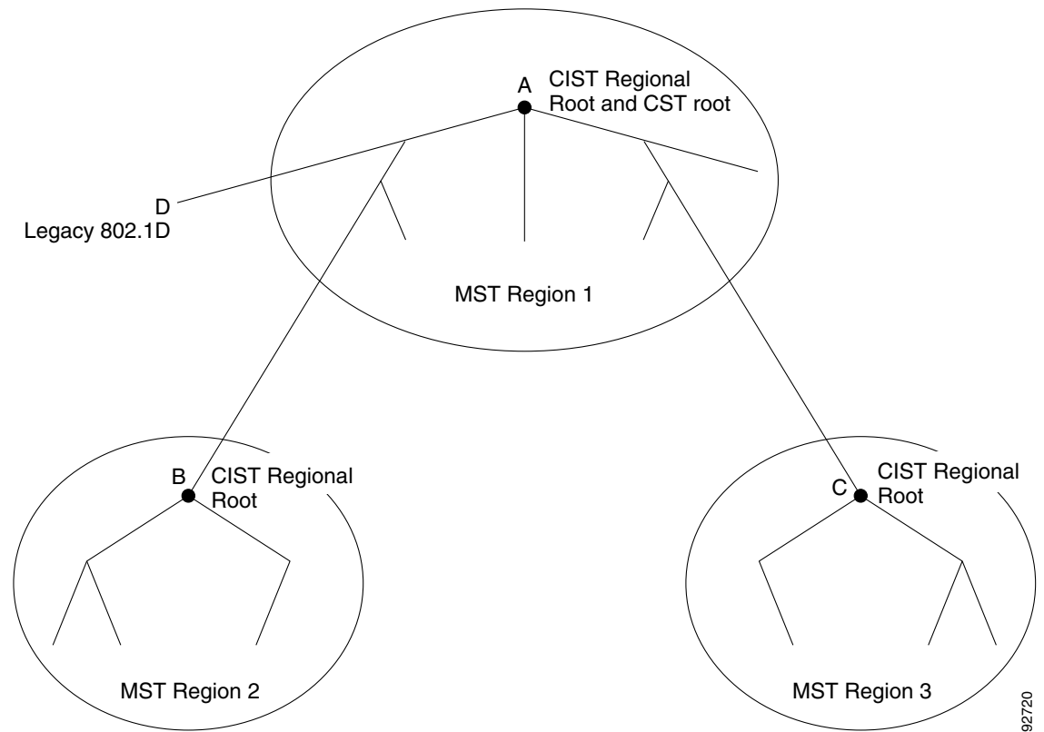
Figure 30-10 MST Regions, CIST Regional Roots, and CST Root
