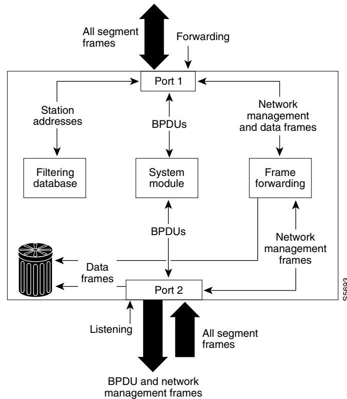
Figure 30-4 Interface 2 in Listening State
