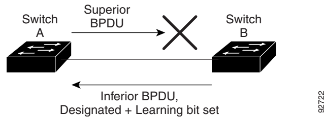
Figure 30-12 Detecting Unidirectional Link Failure
