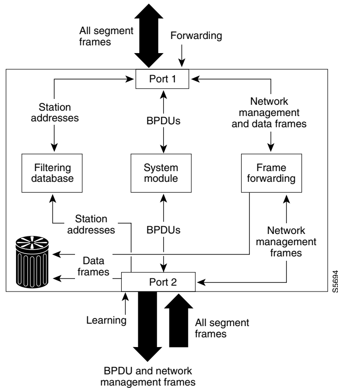
Figure 30-5 Interface 2 in Learning State
