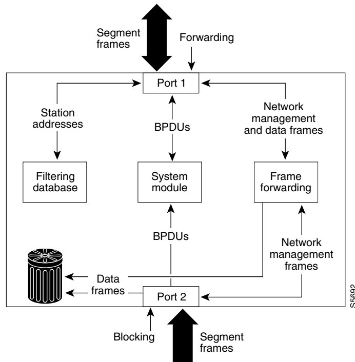
Figure 30-3 Interface 2 in Blocking State
