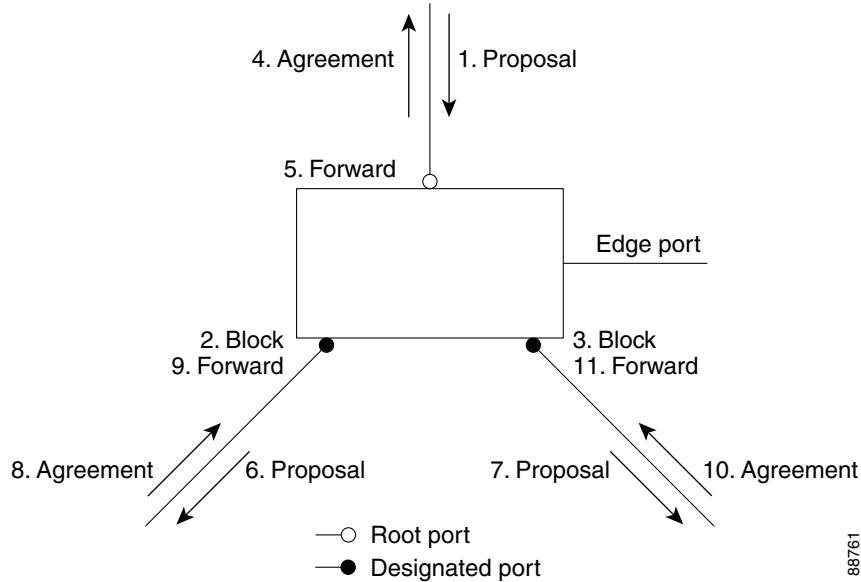
Figure 30-9 Sequence of Events During Rapid Convergence
