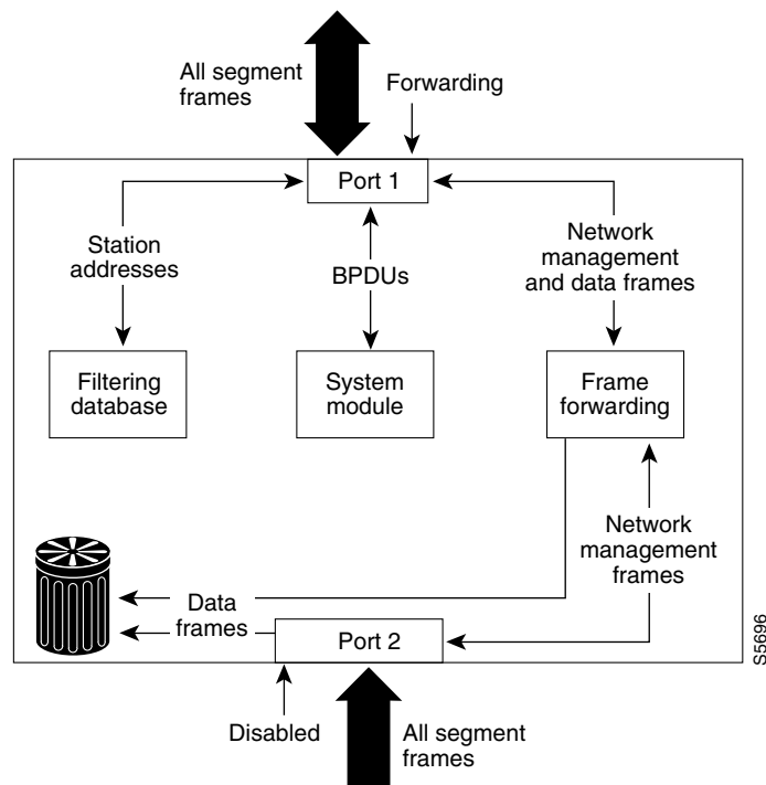
Figure 30-7 Interface 2 in Disabled State
