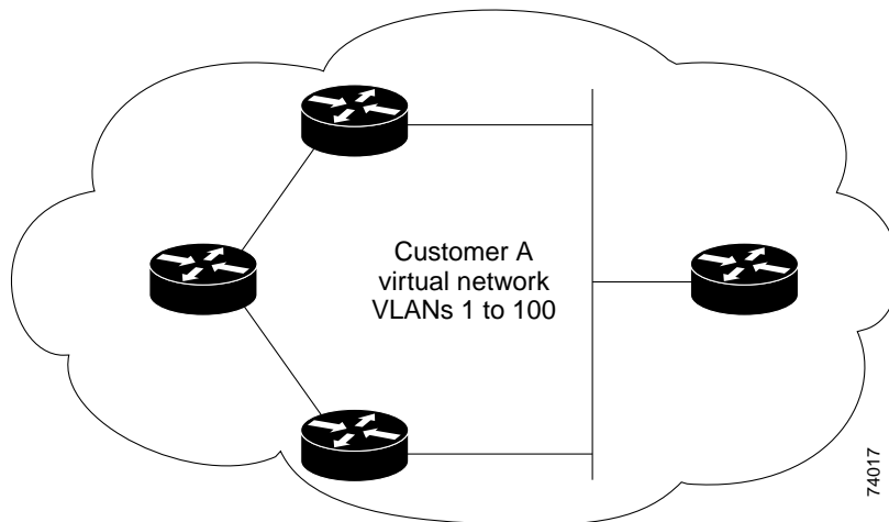
Figure 30-1 802.1Q Tunnel Ports in a Service Provider Network
