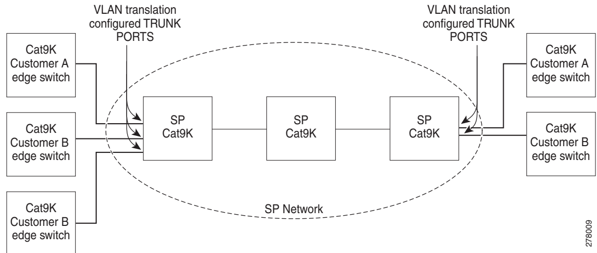
Figure 30-4 Layer 2 VPN Deployment
