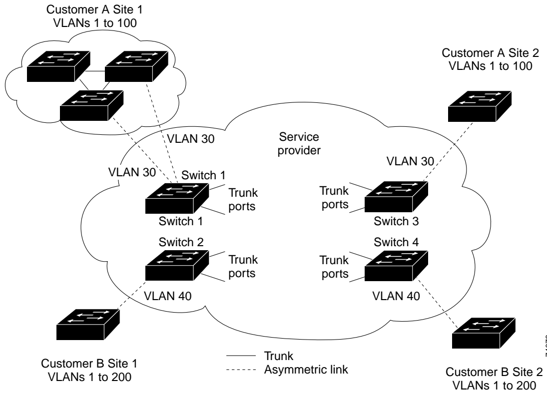
Figure 30-6 Layer 2 Protocol Tunneling
