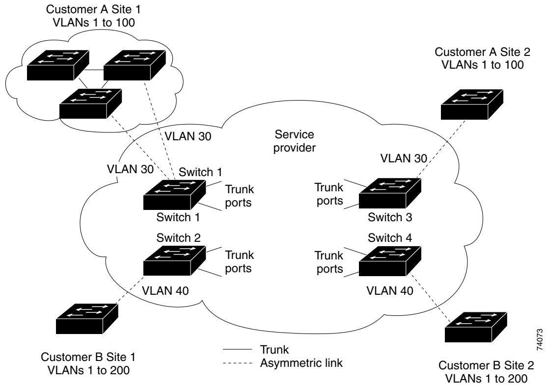
Figure 30-6 Layer 2 Protocol Tunneling
