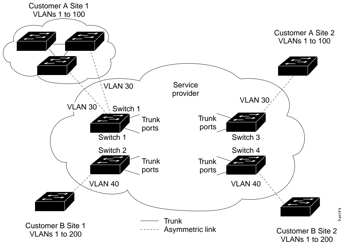
Figure 30-6 Layer 2 Protocol Tunneling
