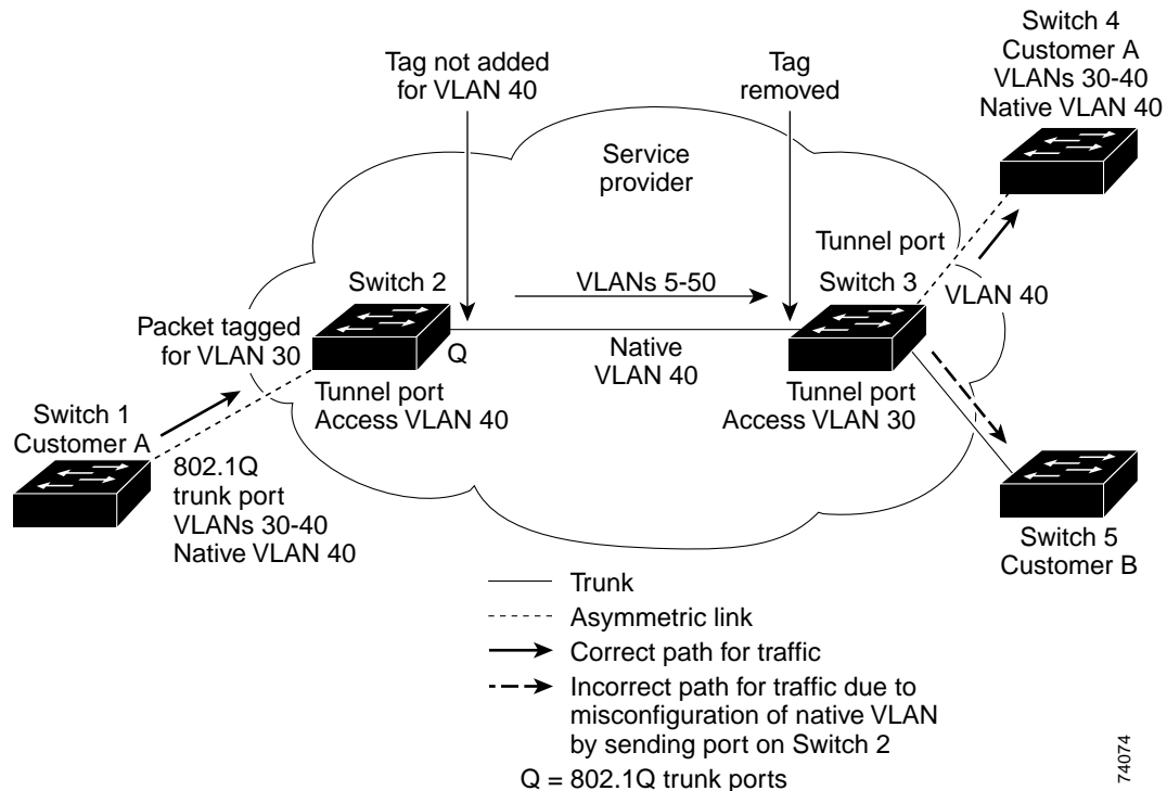
Figure 30-3 Potential Problem with 802.1Q Tunneling and Native VLANs
