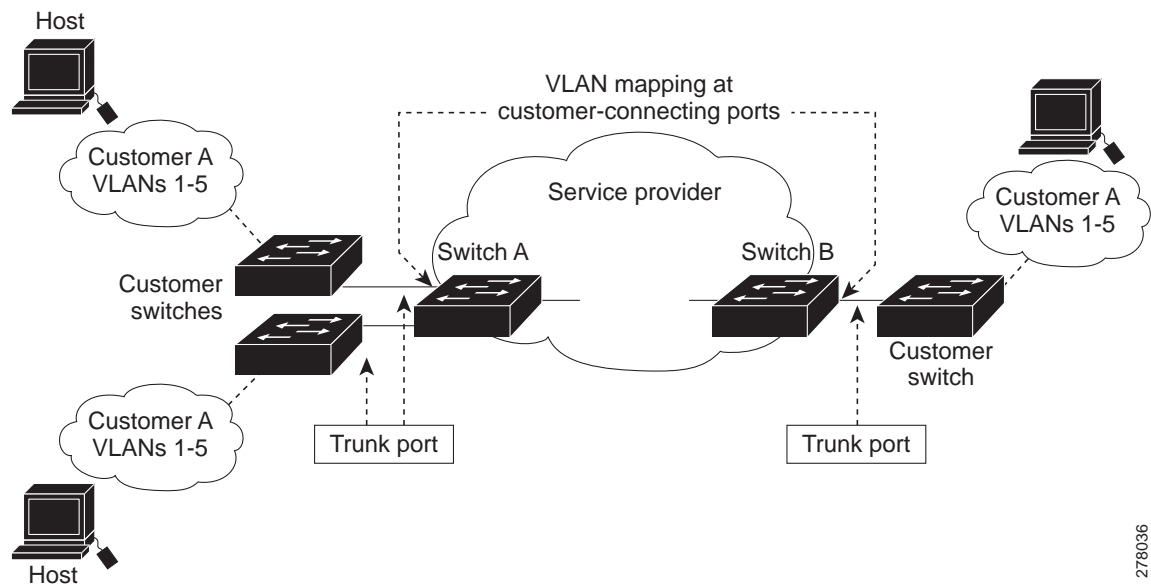
Figure 30-5 Mapping Customer VLANs
