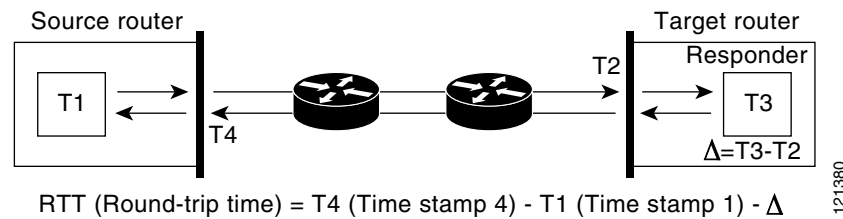
Figure 78-2 Cisco IOS IP SLAs Responder Time Stamping
