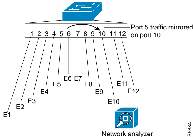
Figure 66-1 Example SPAN Configuration
