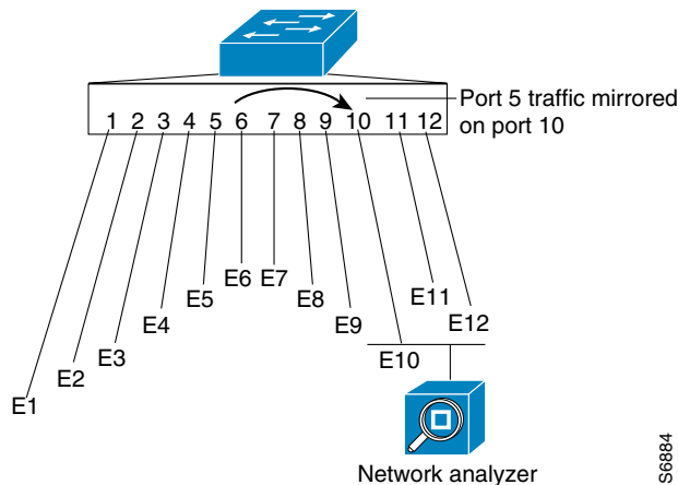
Figure 66-1 Example SPAN Configuration
