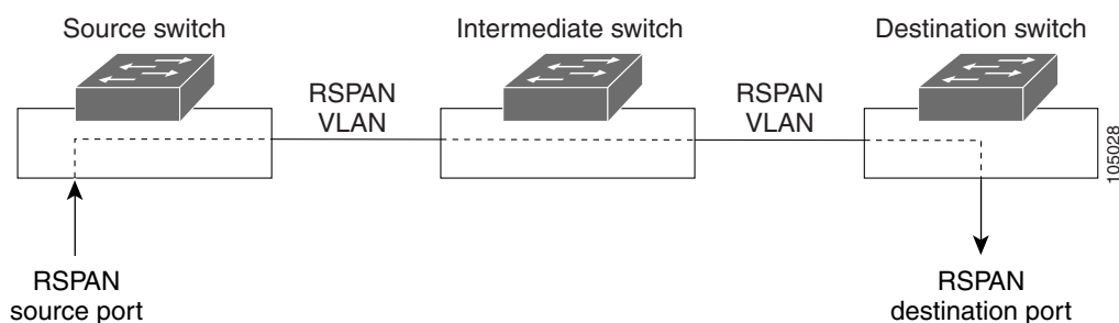
Figure 66-2 Example of RSPAN Configuration
