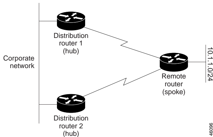
Figure 35-5 Simple Dual-Homed Remote Topology
