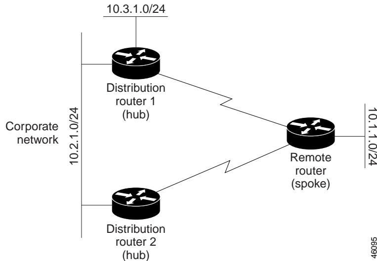
Figure 35-6 Dual-Homed Remote Topology With Distribution Router 1 Connected to Two Networks
