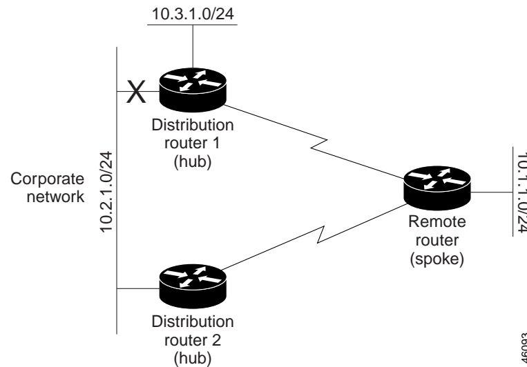
Figure 35-7 Dual-Homed Remote Topology with a Failed Route to a Distribution Router
