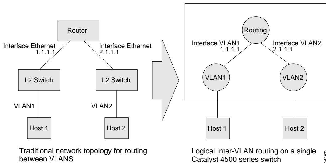
Figure 35-1 Logical Layer 3 VLAN Interfaces for the Catalyst 4500 Series Switch
