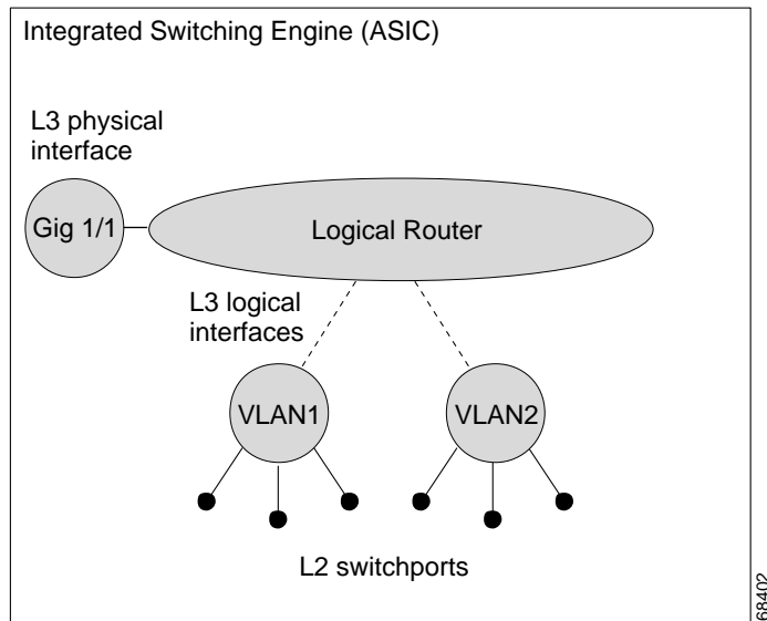
Figure 36-1 Logical L2/L3 Switch Components
