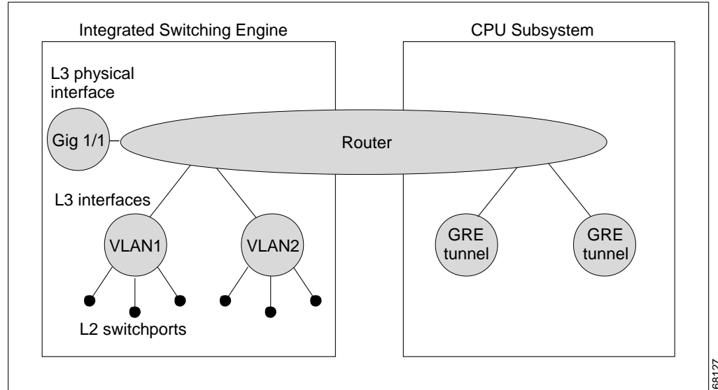
Figure 36-2 Hardware and Software Switching Components
