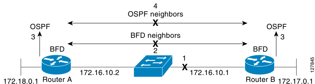
Figure 40-2 Tearing Down an OSPF Neighbor Relationship
