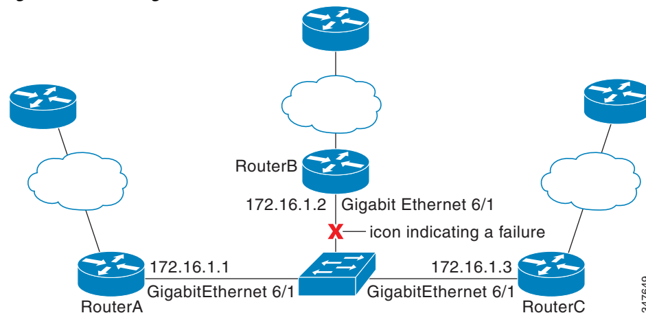
Figure 40-4 Gigabit Ethernet Interface 6/1 Failure
