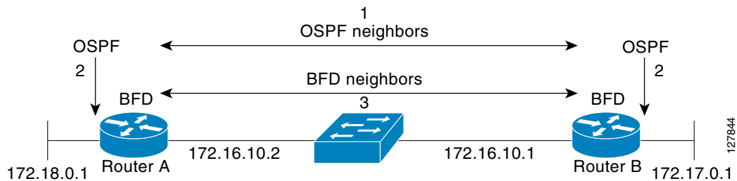
Figure 40-1 Establishing a BFD Neighbor Relationship
