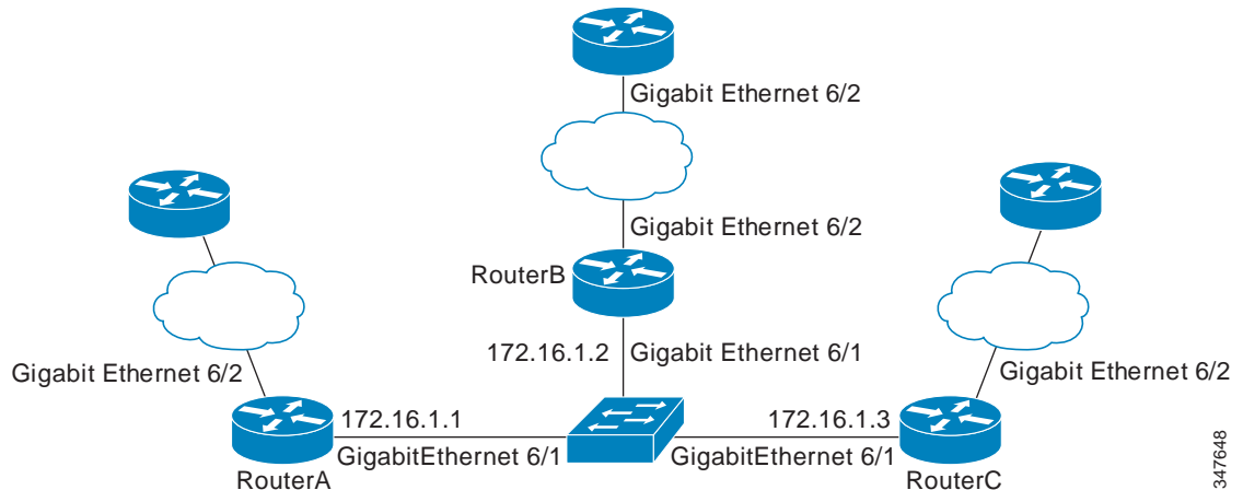
Figure 40-3 EIGRP Network with Three BFD Neighbors Running V1 or V0
