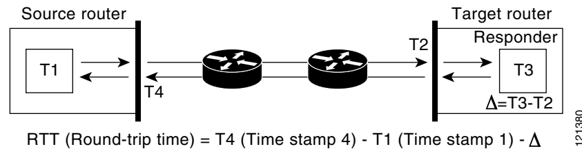
Figure 70-2 Cisco IOS IP SLAs Responder Time Stamping
