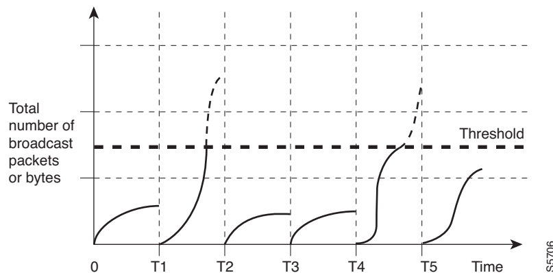
Figure 58-1 Storm Control Example—Hardware-based Implementation
