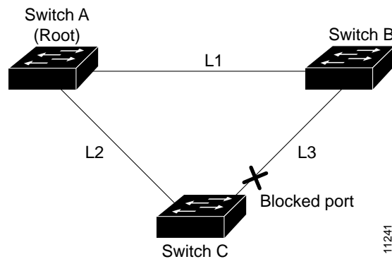
Figure 25-5 BackboneFast after Indirect Link Failure
