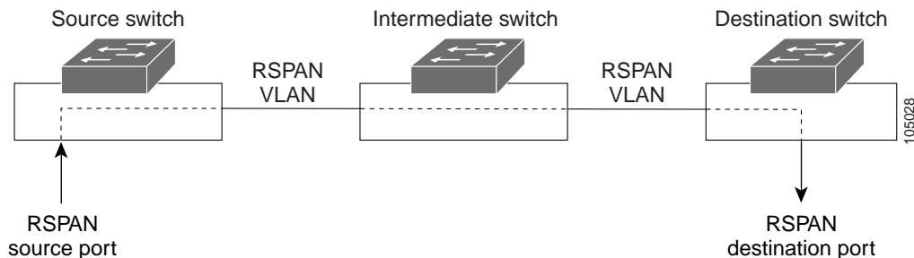
Figure 57-2 Example of RSPAN Configuration
