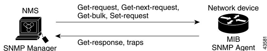
Figure 62-1 SNMP Network
