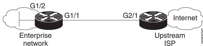
Figure 3-3 Enterprise Network Using Unicast RPF for Ingress Filtering
