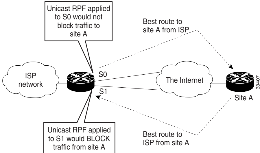
Figure 3-4 Unicast RPF Blocking Traffic in an Asymmetrical Routing Environment
