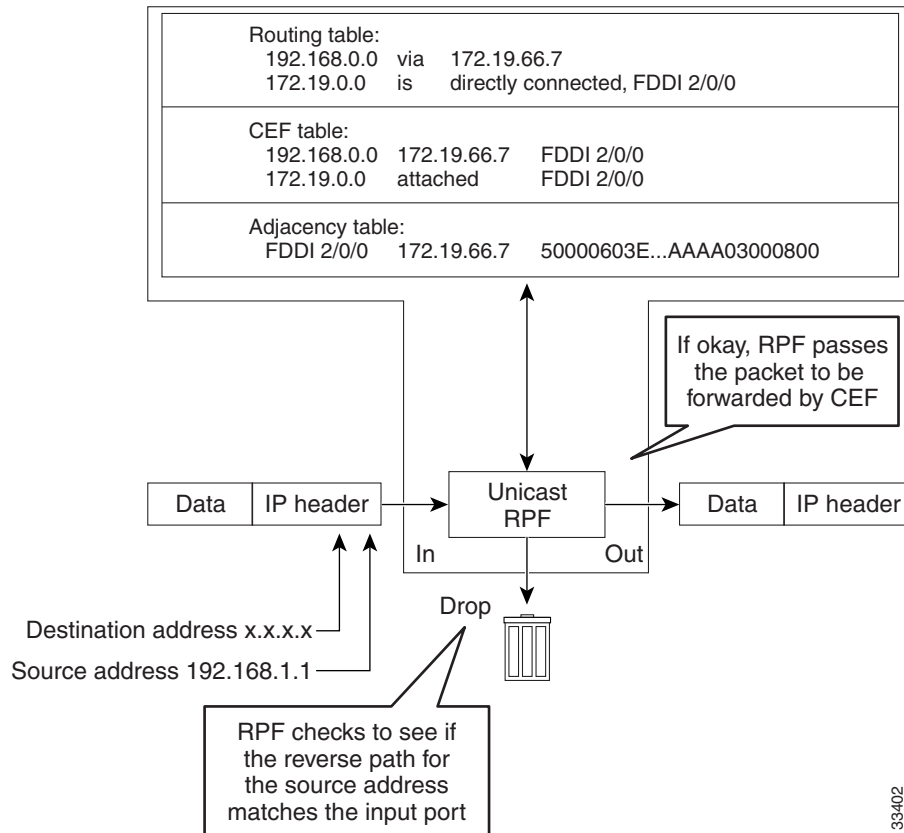
Figure 3-1 Unicast RPF Validating IP Source Addresses
