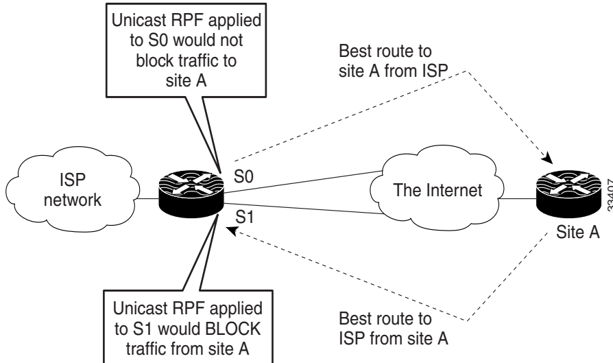
Figure 38-4 Unicast RPF Blocking Traffic in an Asymmetrical Routing Environment
