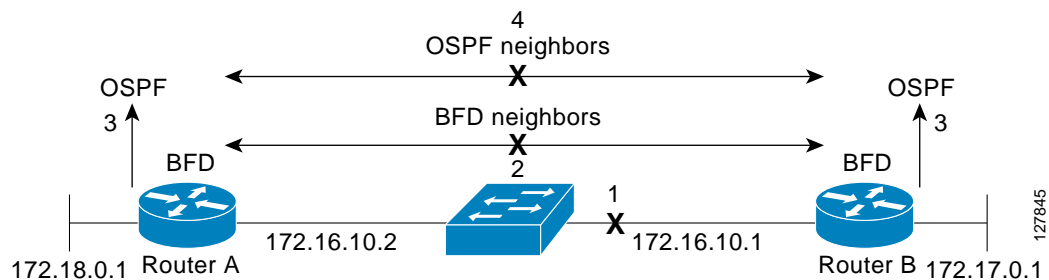
Figure 3-2 Tearing Down an OSPF Neighbor Relationship
