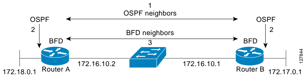
Figure 3-1 Establishing a BFD Neighbor Relationship
