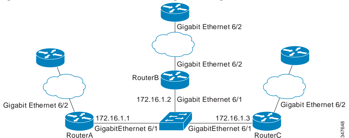
Figure 41-3 EIGRP Network with Three BFD Neighbors Running V1 or V0
