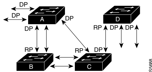
Figure 18-1 Spanning Tree Topology
