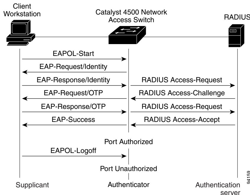
Figure 40-2 Message Exchange
