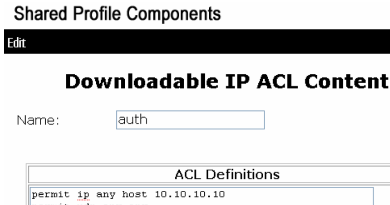
Figure 40-8 Shared Profile Components
