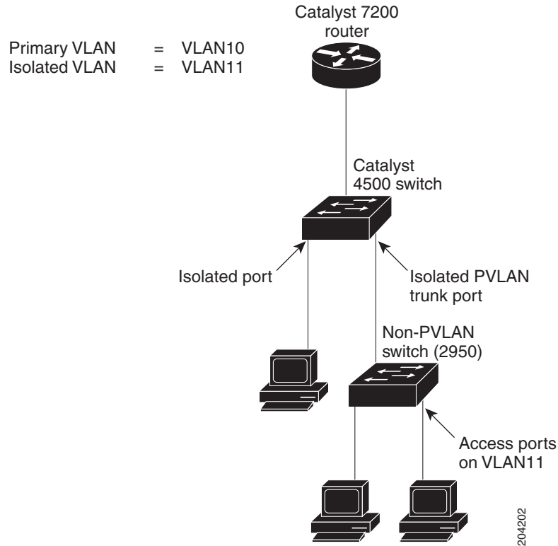
Figure 38-3 Isolated PVLAN Trunk Ports
