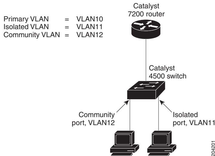
Figure 38-4 Promiscuous PVLAN Trunk Ports
