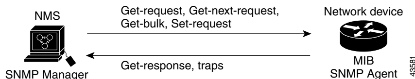
Figure 1-1 SNMP Network
