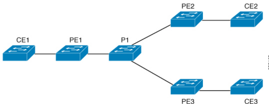
Figure 3: VPLS Topology
