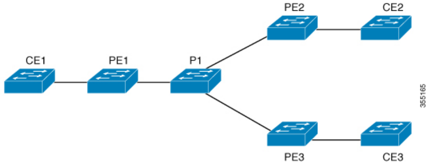
Figure 3: VPLS Topology
