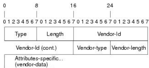
Figure 2: VSA Encapsulated Behind Attribute 26
