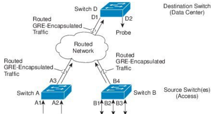
Figure 8: ERSPAN Configuration
