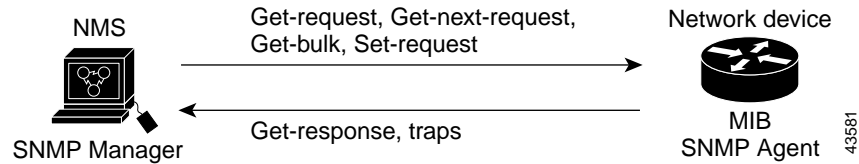
Figure 35-1 SNMP Network
