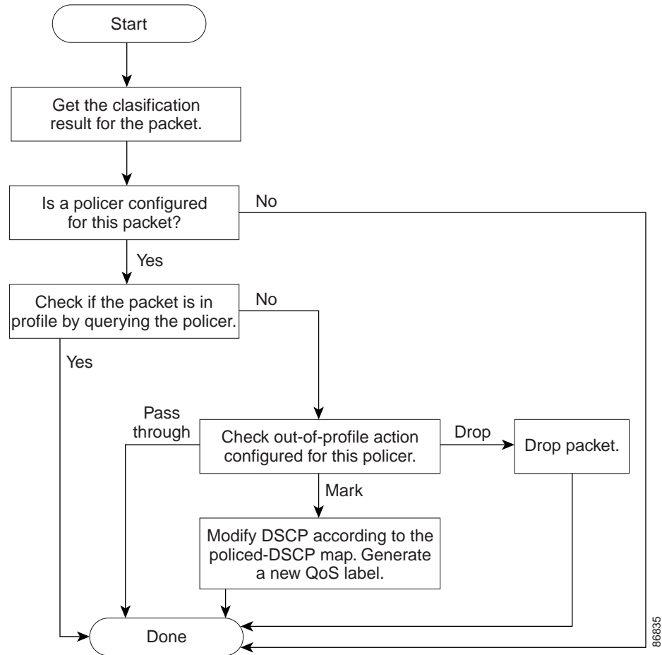
Figure 39-4 Policing and Marking Flowchart on Physical Ports
