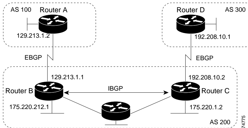
Figure 42-5 EBGP, IBGP, and Multiple Autonomous Systems
