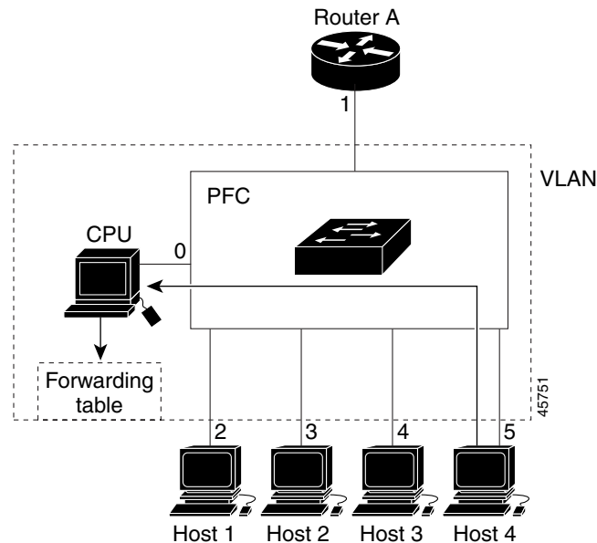
Figure 24-2 Second Host Joining a Multicast Group
