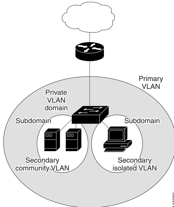
Figure 16-1 Private-VLAN Domain
