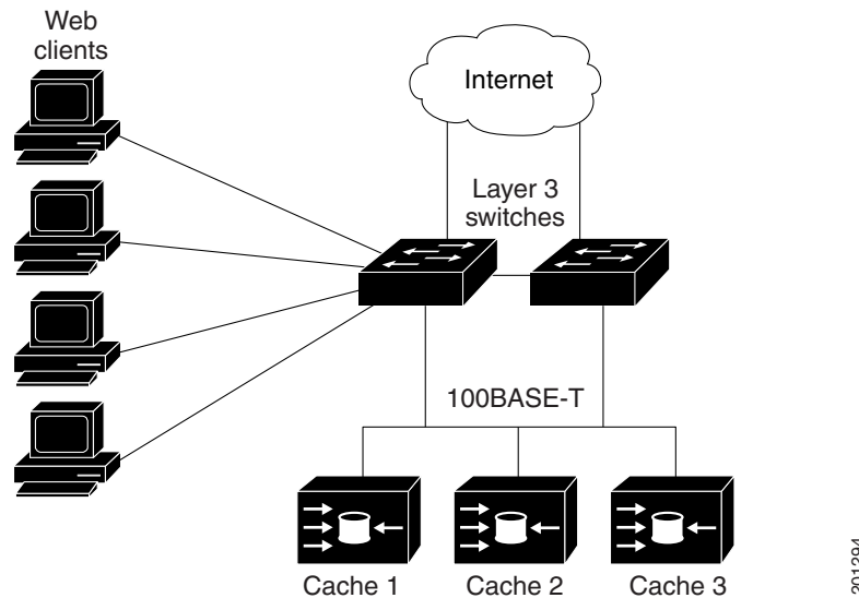
Figure 1-1 Cisco Cache Engine and WCCP Network Configuration
